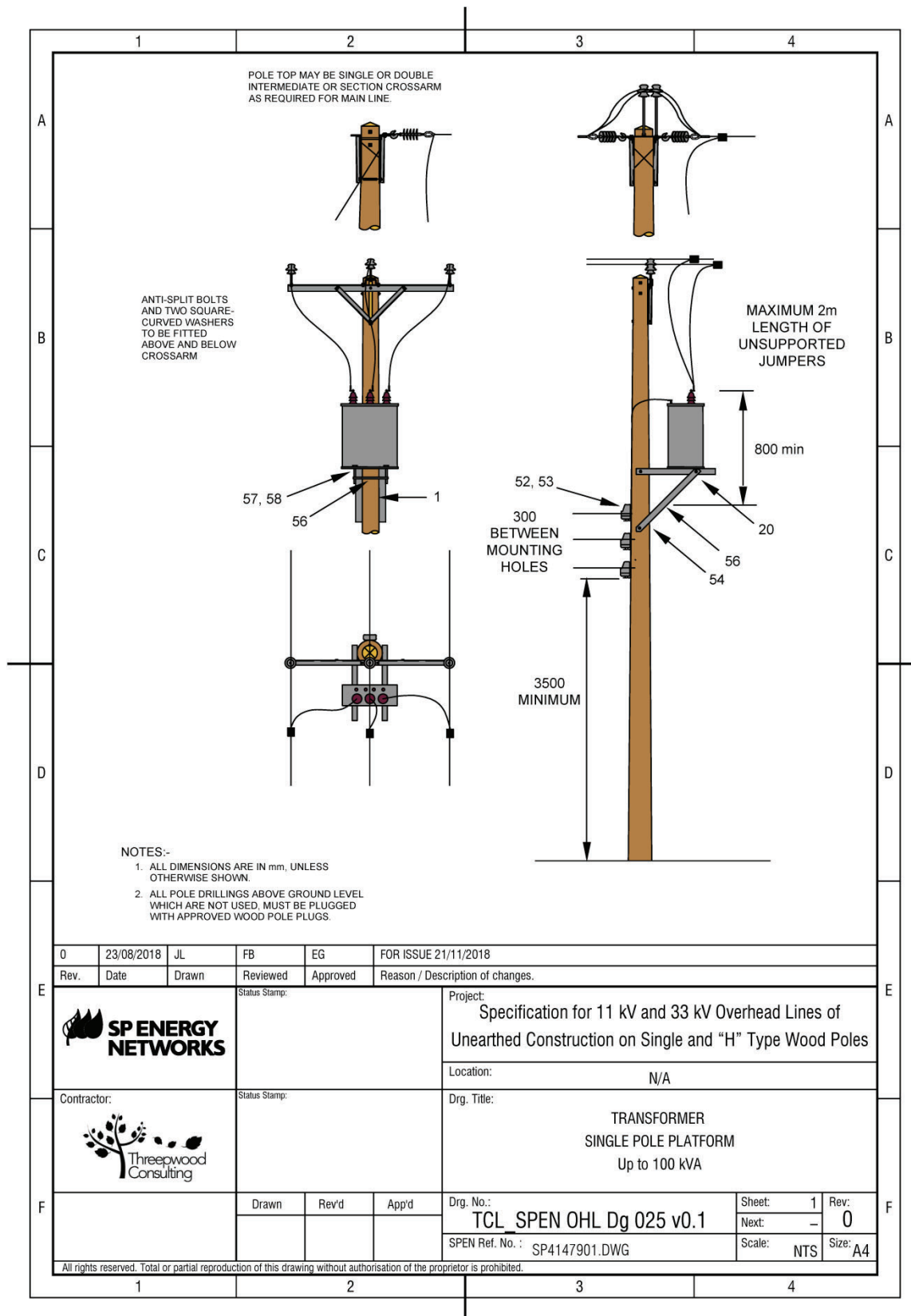
22.25 Figure 25 General Arrangement Transformer Single Pole Platform up to 100kVA (Drawing No. SP4147901)
